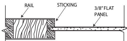
Shaker Square Sticking
