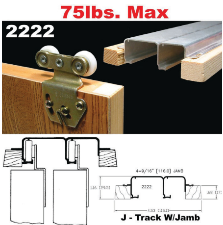
POCKET DOOR HARDWARE
