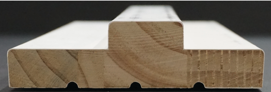
DOUBLE RABBETED JAMBS
