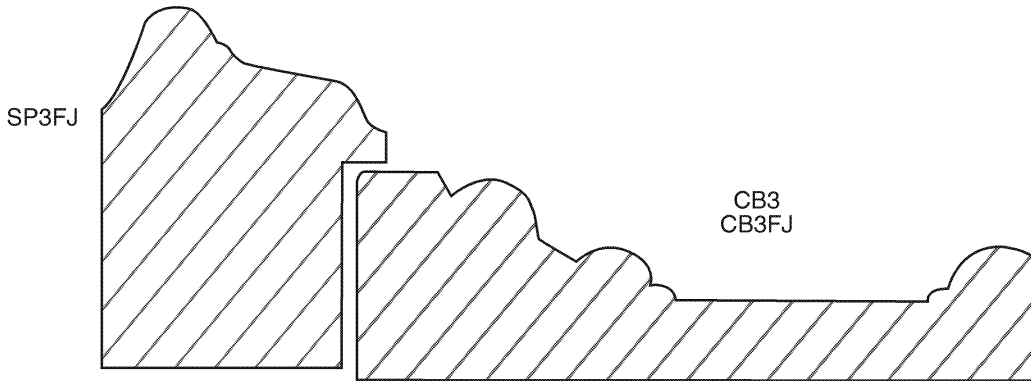
CB SP3 383 1 X 1 7/8" BACK BAND FJ PINE
