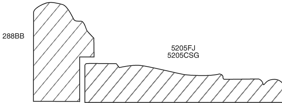
CB 288 11/16" X 1 5/8" BACK BAND A GRADE PINE
