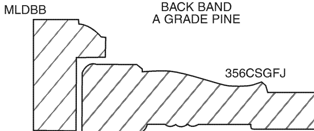
CB 281 11/16" X 1 1/8" BACK BAND A GRADE PINE
