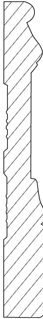
CB 616 11/16" X 5 1/4" VICTORIAN BASE FJ PINE
