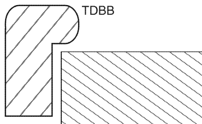
CB 280 11/16" X 1 1/8" BACK BAND A GRADE PINE
