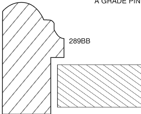
CB 289 1 1/8" X 2" BACK BAND A GRADE PINE
